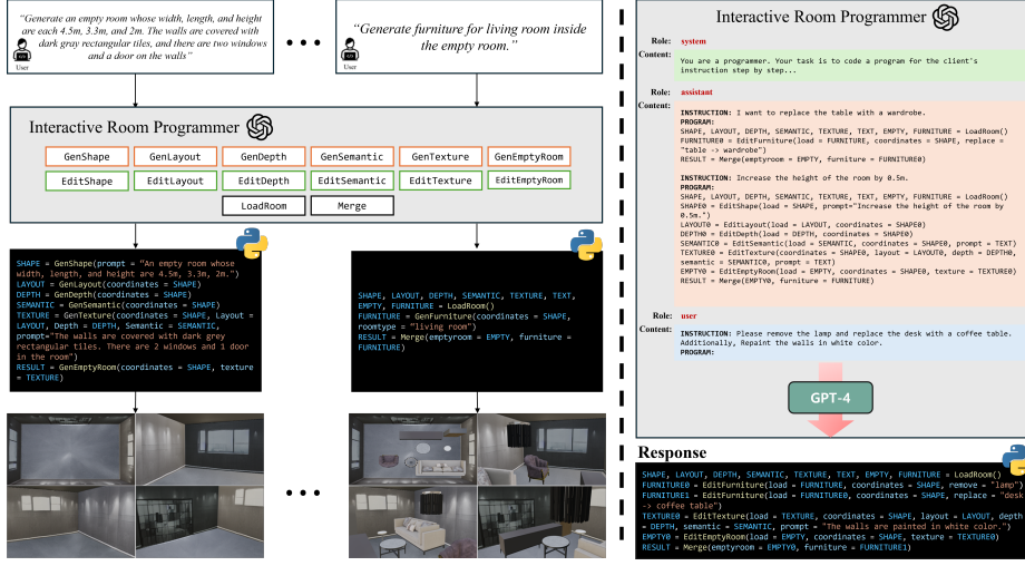
Fig. 2: (left) Overall pipeline. IRP converts a user-provided instruction into a Python program of predefined modules. Users can continuously edit the generated room until they obtain the most satisfying result. (right) Prompts given to an LLM, including supporting examples for in-context-learning are illustrated.
