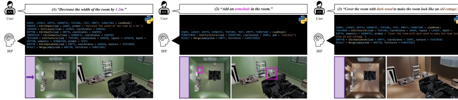
Fig. 1: Editing examples supported by IRP. Pairs of user instructions and corresponding bounding boxes are illustrated in the same color.
